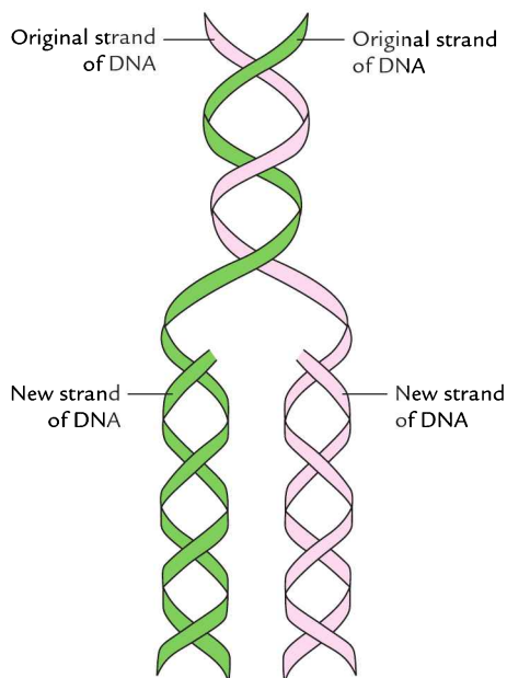
Fig. 17.2 DNA replication.
